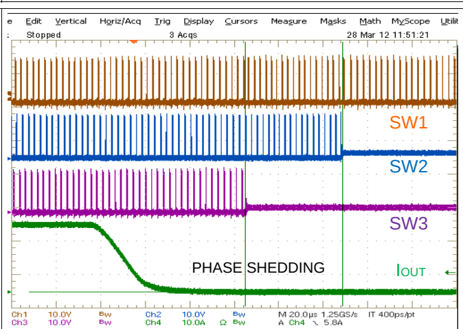
Figure 116. Phase Shedding
