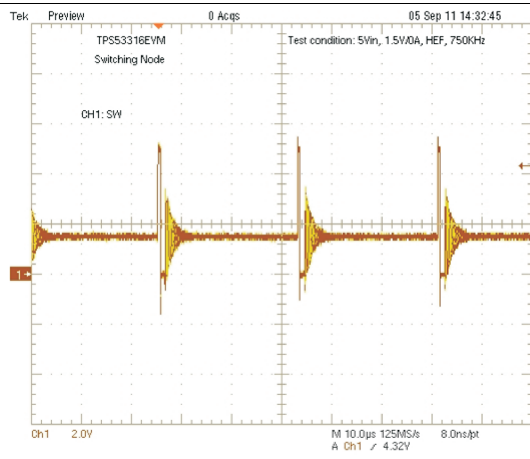
5-V VIN, 1.5-V VOUT, 0-A, HEF Mode, and f_{SW} = 750 kHz Figure 48. Switching Node
