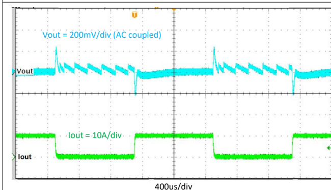
Figure 8-16. Transient Response, 0 A to 10 A, Slew Rate = 2.5\text{ A}/\mu\text{s}
