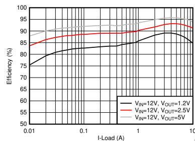
Efficiency vs Output Current, 500 kHz, Eco-mode
