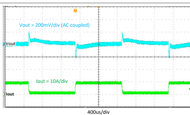
Figure 8-15. Transient Response, 1 A to 9 A, Slew Rate = 2.5\text{ A}/\mu\text{s}
