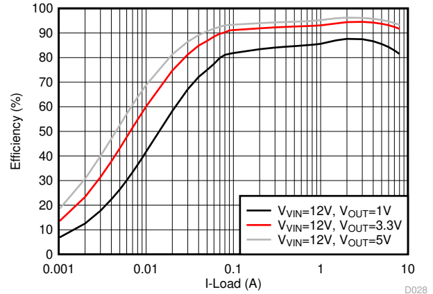
Figure 6-14. Efficiency, OOA-mode, F_{SW} = 600 kHz
