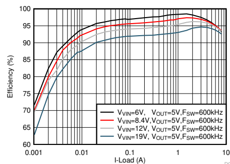
Efficiency vs Output Current ECO-mode
