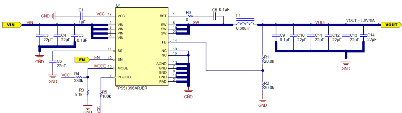
Figure 8-1. 1V/8A Reference Design with Eco-mode, Fsw = 600 kHz
