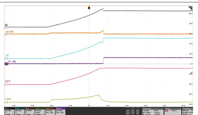
Figure 8-12. Inrush Current Profile With 220 \mu F at the Output and 0.5A Load (LPM = Low)
