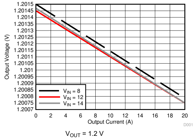
Figure 9-3. Line Regulation
