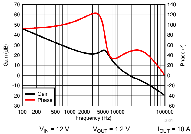
Figure 9-4. Bode Plot
