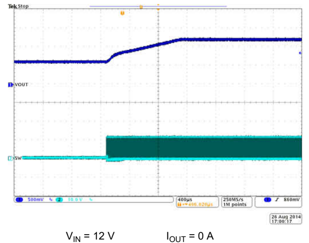
Figure 9-5. Prebias Start-Up
