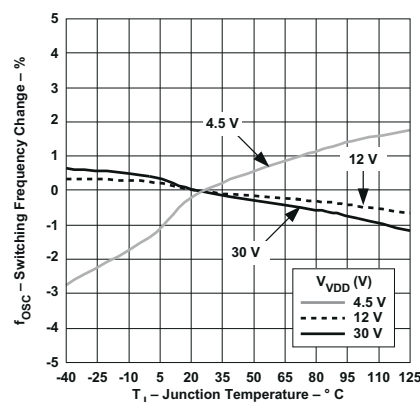
Figure 6-10. Switching Frequency Change vs Junction Temperature
