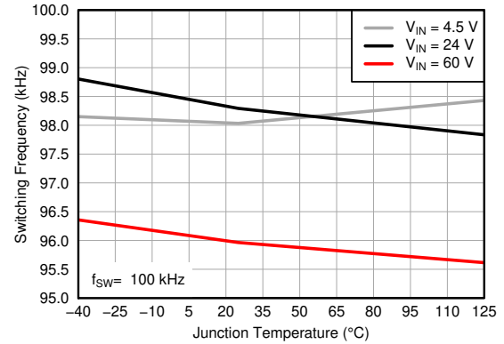
Figure 5-2. Switching Frequency vs Junction Temperature
