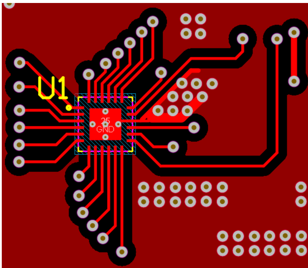
Figure 8-7. Recommended Layout
