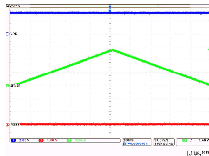
Figure 26. TPS3870-Q1 SENSE Ramp Latch Function
