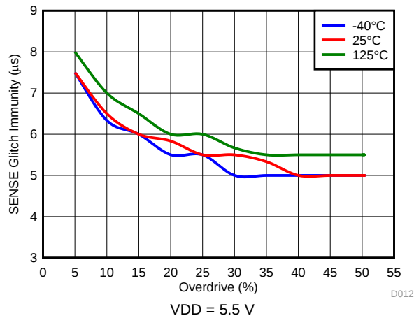
Figure 9. SENSE Glitch Immunity (VIT+) vs Overdrive
