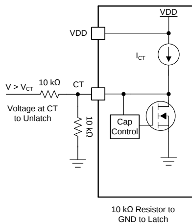
Figure 22. RESET Latch Circuit
