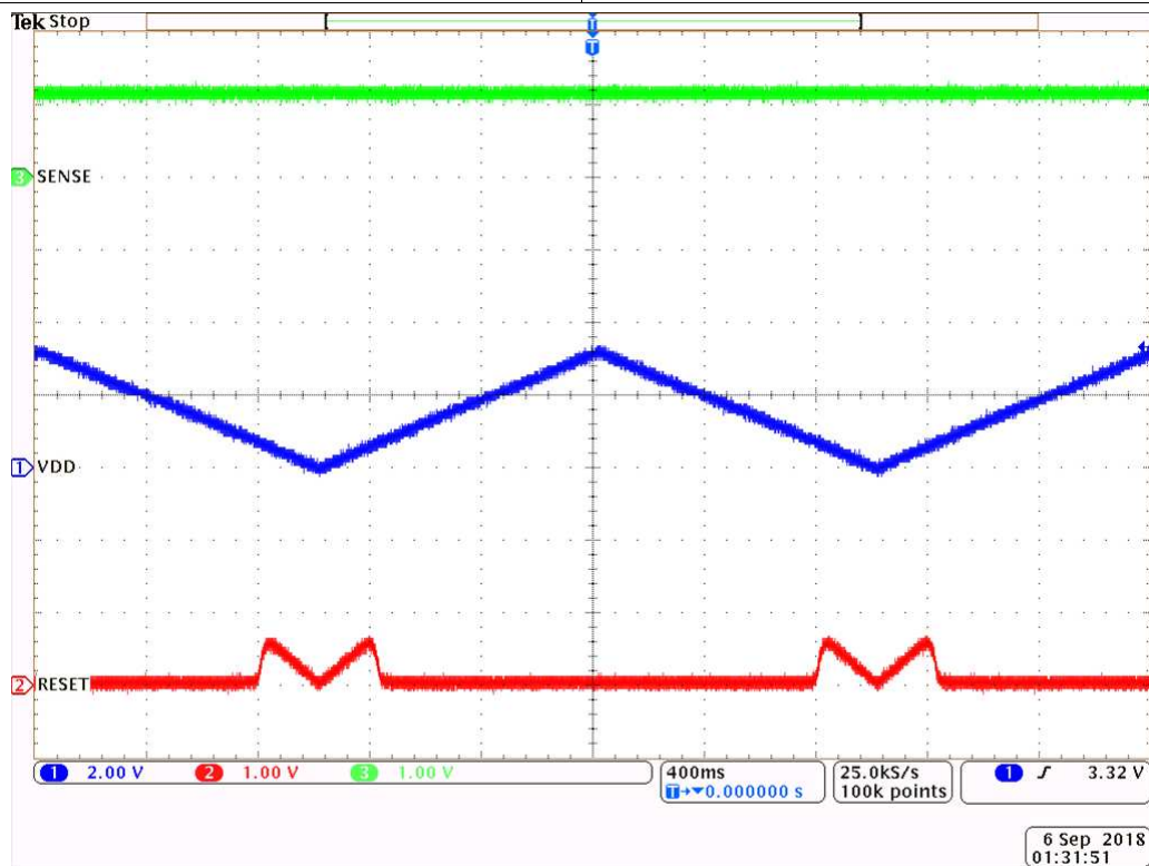
Figure 26. TPS3870-Q1 SENSE Ramp Latch Function
