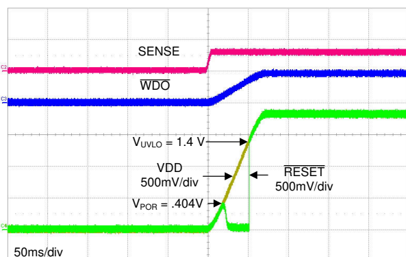
Figure 8-7. Startup Waveform
