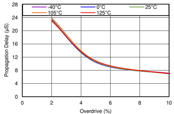
Figure 5-9. Overvoltage Propagation Delay vs Overdrive
