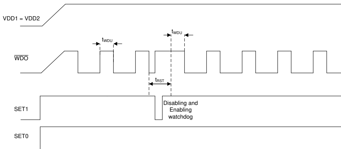
Figure 7-3. Enabling and Disabling the Watchdog Timer During a WDO Reset Event
