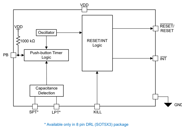
Figure 7-3. TPS3424 Block Diagram (Active Low Push-Button Input)
