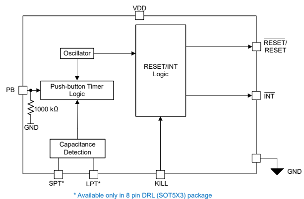
Figure 7-4. TPS3424 Block Diagram (Active High Push-Button Input)
