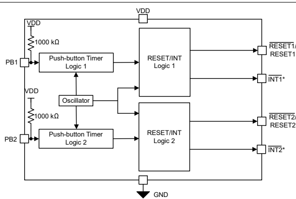
Figure 7-1. TPS3423 Block Diagram (Active Low Push-Button Input)
