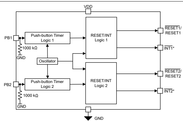
Figure 7-2. TPS3423 Block Diagram (Active High Push-Button Input)
