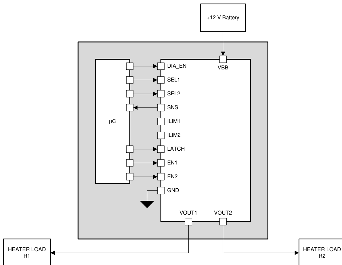
Figure 46. Block Diagram for Powering Dual Heater Loads
