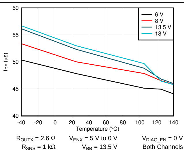
Figure 12. Turn-off Delay Time ( t_{DF} ) vs Temperature
