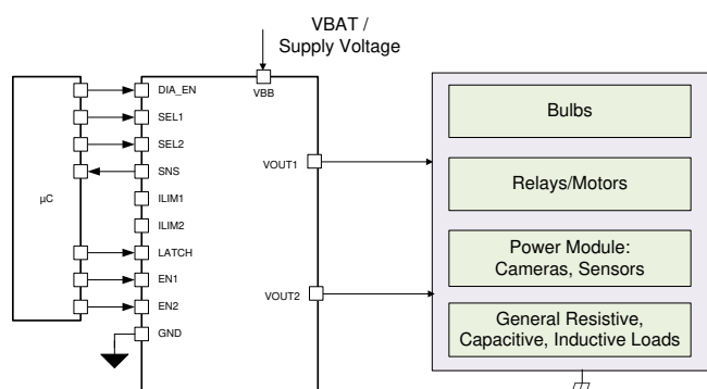
Simplified Schematic
