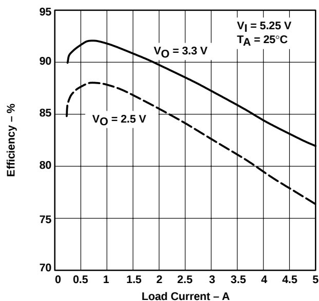
Figure 26. Converter Efficiency
