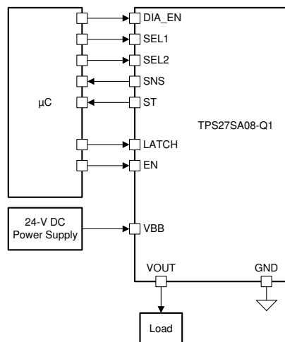
Simplified Schematic
