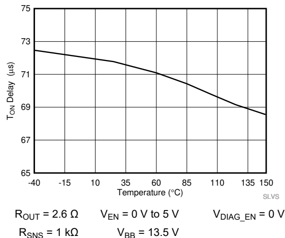
Figure 7-7. Turn-on Delay Time ( t_{DR} ) vs Temperature
