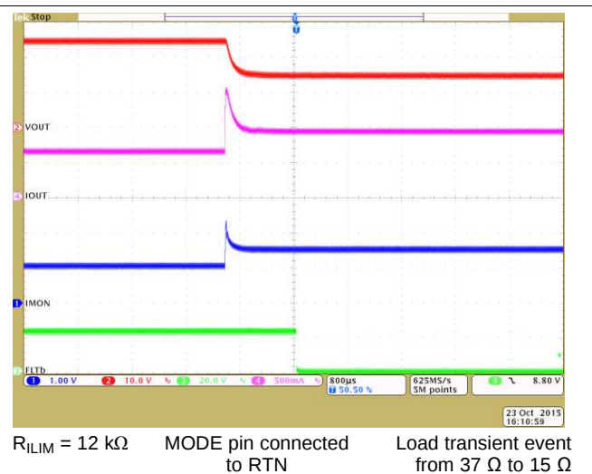
Figure 47. Output Turnoff Due to Thermal Shutdown With FLT Asserted in Advance
