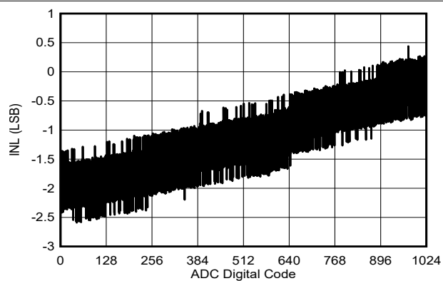
Figure 7-24. ADC INL
