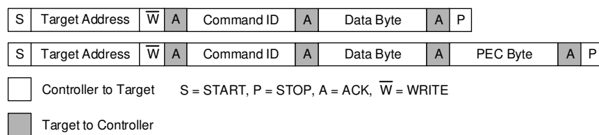
Figure 8-12. Write Byte
