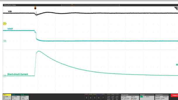
Figure 9-13. Output Hot-Short Response: V_{IN} = 12\text{ V} , R_{IMON} = 150\text{ }\Omega , V_{IREF} = 1\text{ V} , and OUT Shorted to GND
