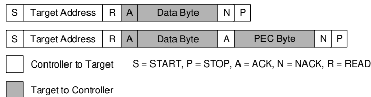
Figure 8-11. Receive Byte
