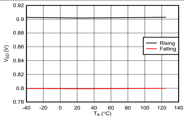
Figure 7-10. EN/UVLO Based Shutdown Thresholds Across Temperature
