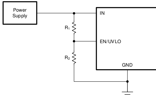
Figure 8-2. Adjustable Undervoltage Protection
