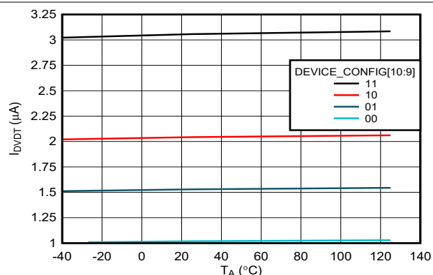
Figure 7-22. DVDT Pin Charging Current Across Temperature
