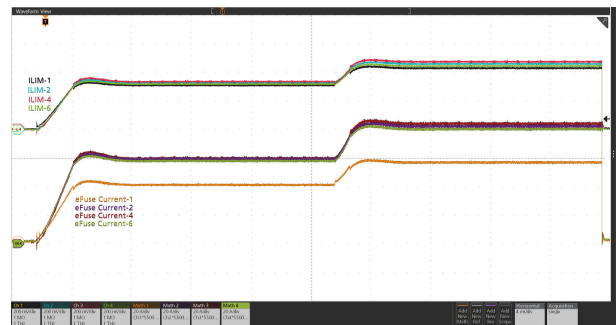
Figure 9-12. Circuit-Breaker Response (Current distribution among six devices in parallel): V_{IN} = 12\text{ V} , t_{OC\_TIMER} = 17\text{ ms} , C_{LOAD} = 50\text{ mF} , R_{IMON} = 150\text{ }\Omega , V_{IREF} = 1\text{ V} , and Load Current Stepped from 333 A to 530 A for more than 17 ms
