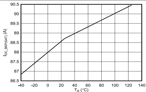
Figure 7-20. Backup Overcurrent Protection Threshold (Startup) Accuracy
