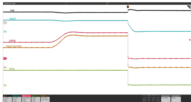
Figure 9-11. Circuit-Breaker Response: V_{IN} = 12\text{ V} , t_{OC\_TIMER} = 10\text{ ms} , C_{LOAD} = 50\text{ mF} , R_{IMON} = 150\text{ }\Omega , V_{IREF} = 1\text{ V} , and Load Current Stepped from 333 A to 530 A for more than 10 ms
