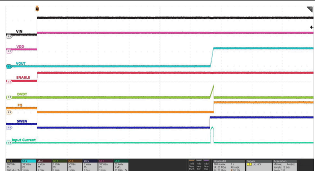
Figure 7-36. Input Hot Plug
