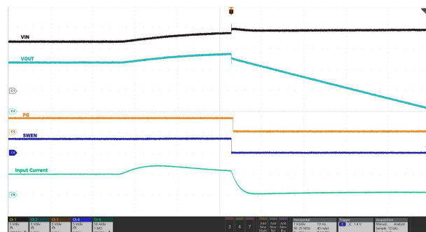
Figure 7-44. Input Undervoltage Protection
