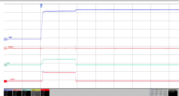
Figure 9-15. Power Up with Short Circuit on Output
