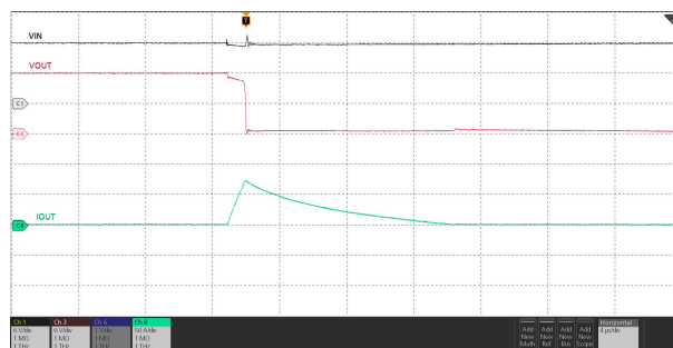
Figure 7-35. Circuit-Breaker Response
