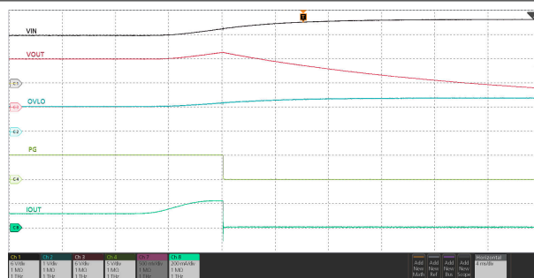
Figure 7-33. Overvoltage Lockout Response
