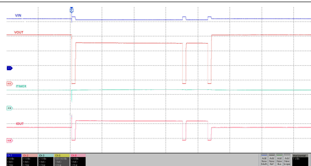
Figure 9-13. Overload Response and Recovery
