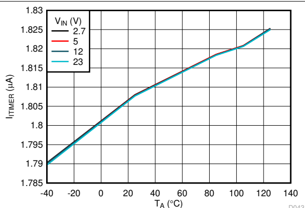
Figure 7-29. ITIMER Discharge Current vs Temperature
