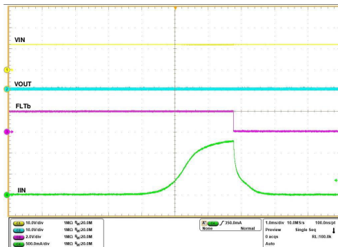
Figure 7-53. Output Short-Circuit During Steady State
