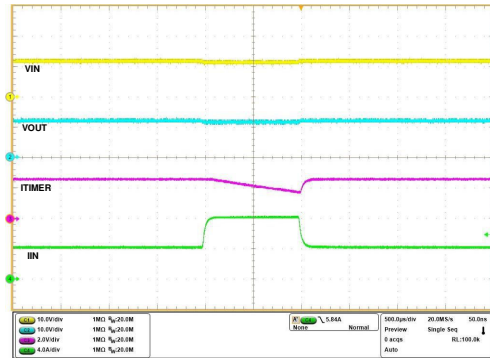
Figure 7-51. Transient Overcurrent Blanking Timer Response - TPS259474x
