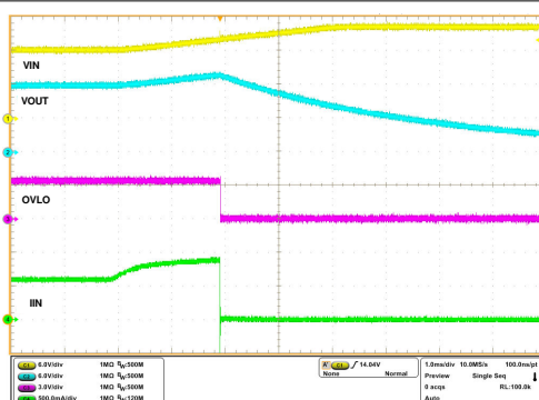
Figure 7-45. Overvoltage Lockout Response - TPS259470x/4x
