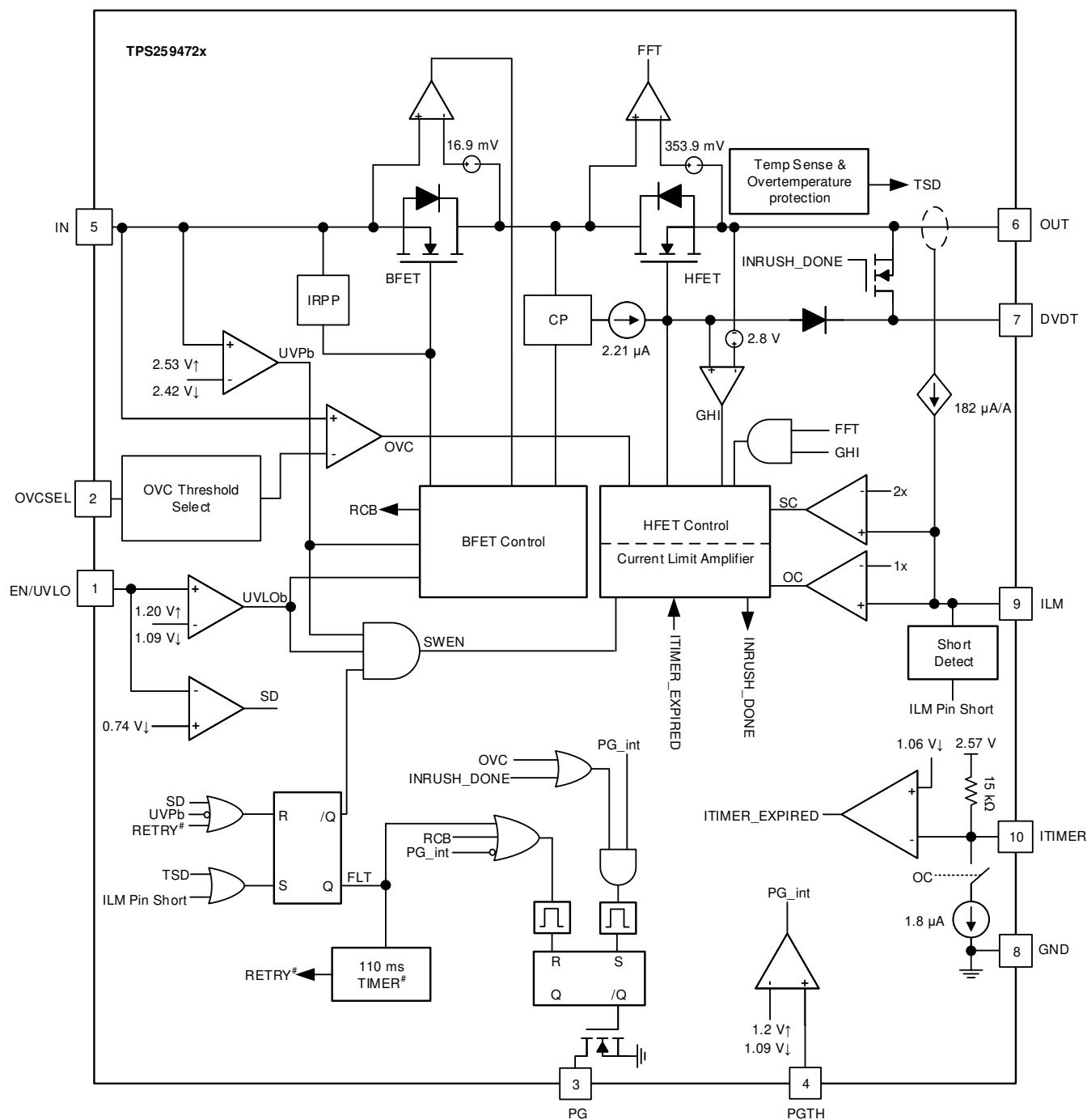
Figure 8-2. TPS259472x Block Diagram
