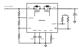
Simplified Schematic
