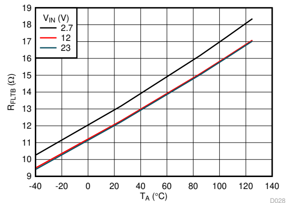
Figure 7-35. FLTB Pin Pulldown Resistance vs Temperature
