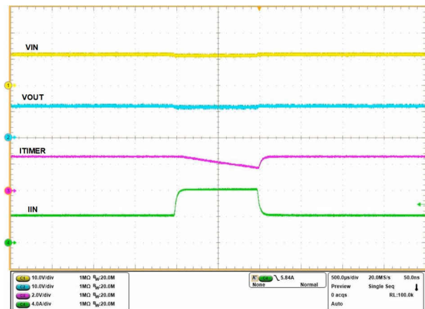
Figure 9-5. Transient Overload
