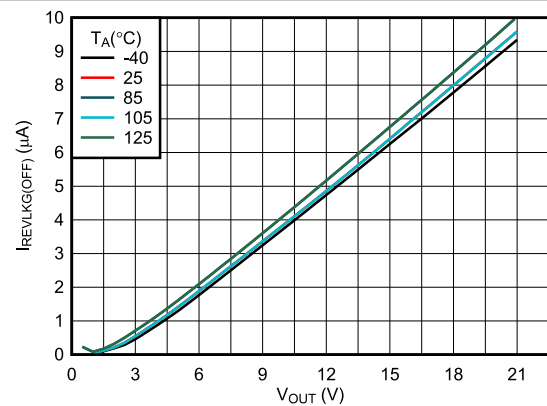
Figure 7-23. Reverse Leakage Current During OFF-State
