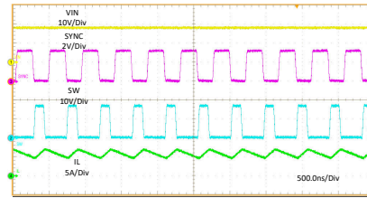
Figure 10-10. Synchronizing to External 2.2-MHz Clock
