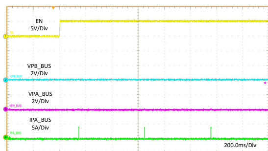
Figure 11-20. Rd Assert
