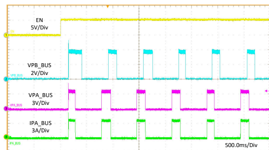
Figure 11-22. Enable Into Short
