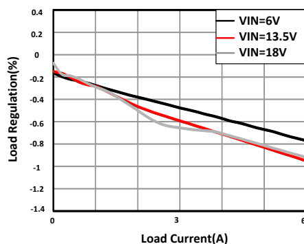
Figure 11-5. Load Regulation
