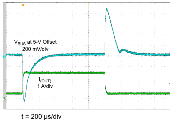
Figure 9-8. 0.5-A \leftrightarrow 2.4-A Load Transient With 100-mA/ \mu s Slew Rate, V_{BUS}
