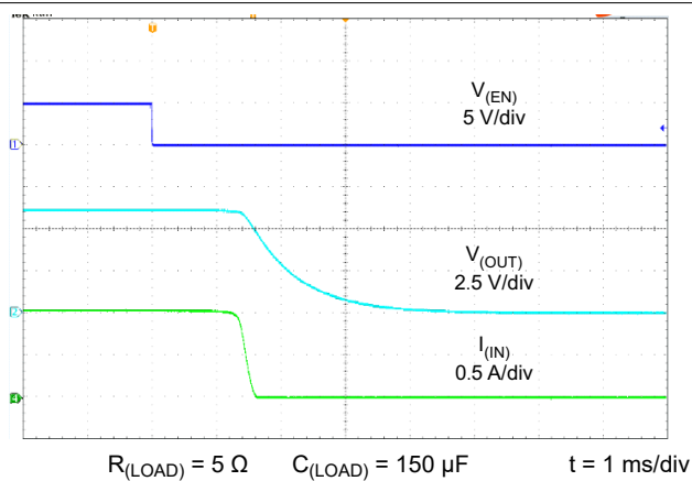
Figure 6-21. Turnoff Response
