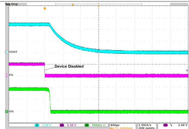
Figure 6. Turnoff Delay and Fall Time
