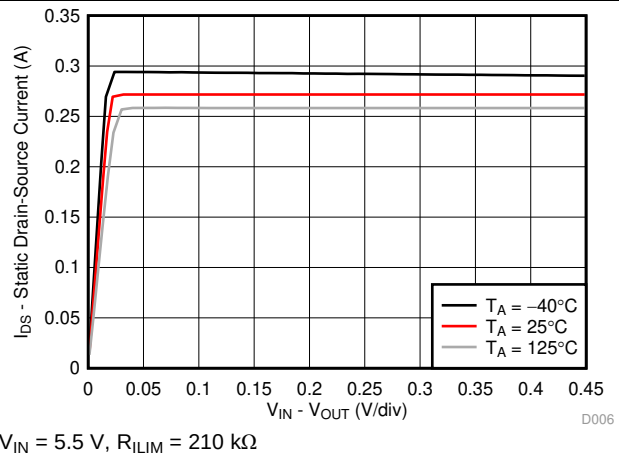
Figure 20. Switch Current Vs. Drain-Source Voltage Across Switch
