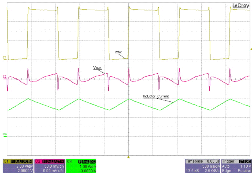
Figure 29. V AUX Ripple, V IN = 3.3 V, I AUX = 1 A
