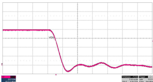
Figure 8-9. Slew Rate Adjust SRF = 0 Ω
