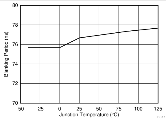
Figure 6-16. Blanking Period vs Temperature
