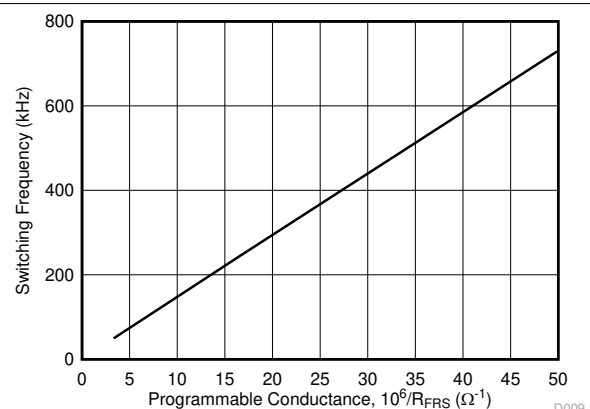
Figure 6-10. Switching Frequency vs Programmed Resistance
