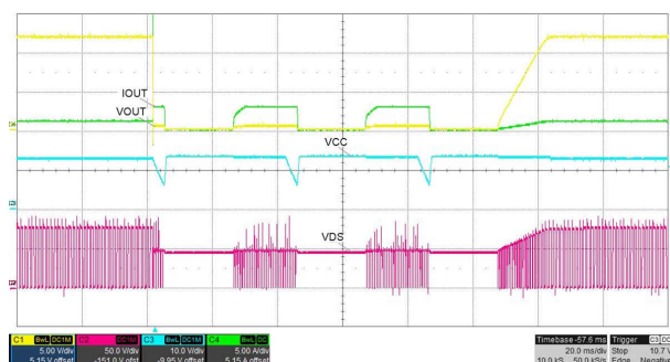
Figure 8-6. TPS23755 Output Short and Recovery
