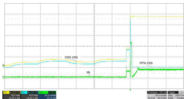
Figure 8-4. TPS23755 Startup to TPS23861 PSE
