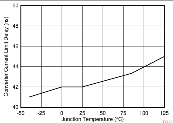
Figure 6-18. Converter Current Limit Delay vs Temperature
