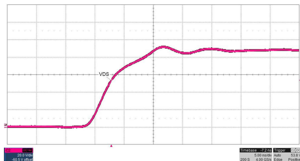
Figure 8-8. Slew Rate Adjust SRR = 0 Ω
