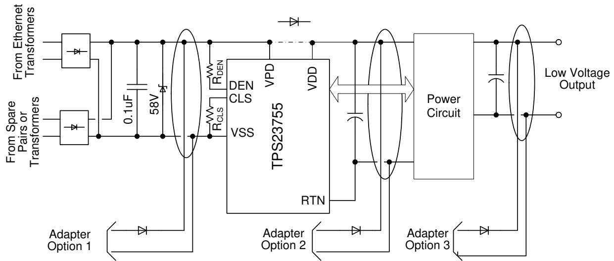
Figure 7-11. ORing Configurations
