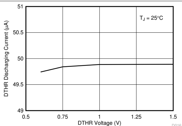
Figure 6-12. Frequency Dithering Discharging Current
