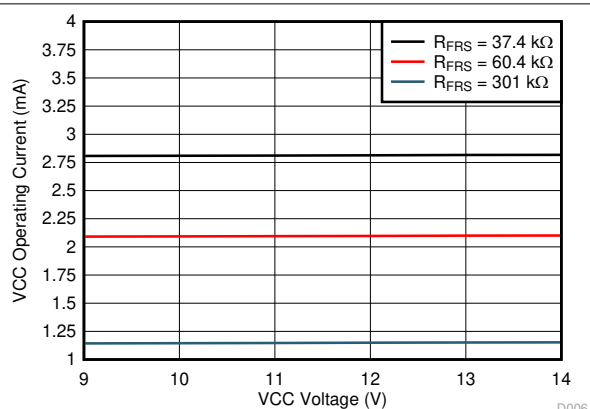
Figure 6-8. Controller Bias Current vs Voltage
