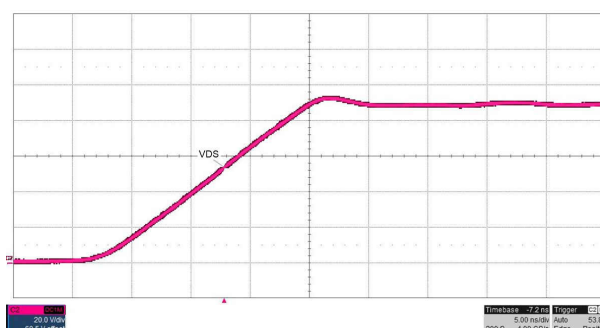
Figure 8-7. Slew Rate Adjust SRR = 15 Ω
