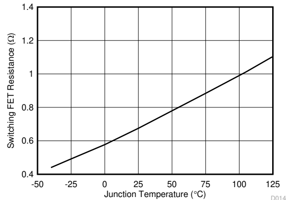
Figure 6-23. Switching FET Resistance vs Temperature
