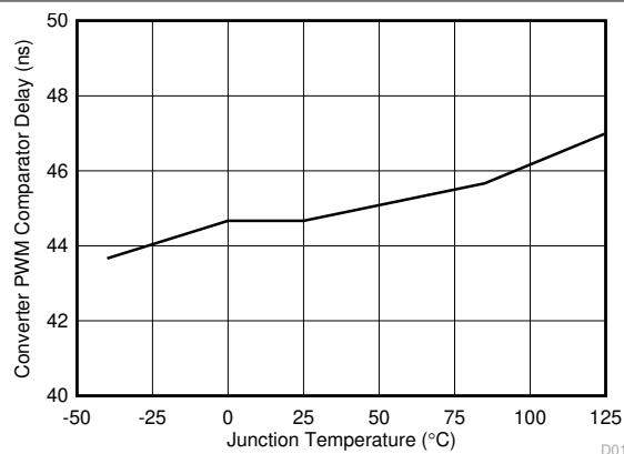
Figure 6-17. Converter PWM Comparator Delay vs Temperature
