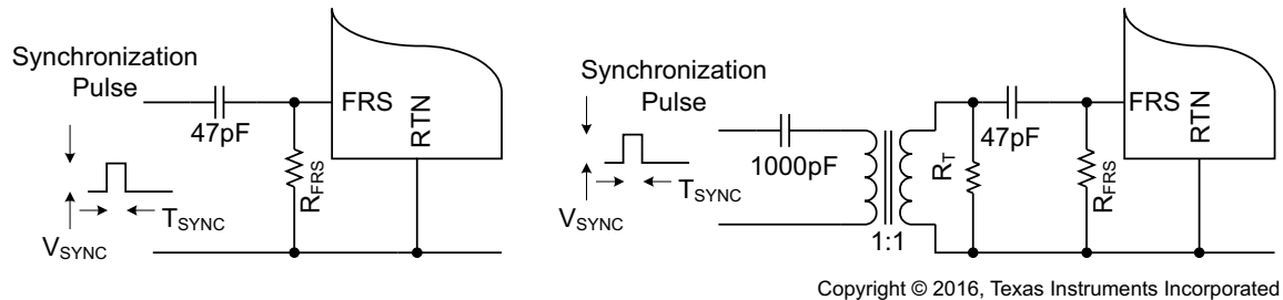
Figure 7-3. Synchronization
