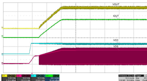
Figure 8-5. TPS23755 PSR Flyback Startup to Full Load
