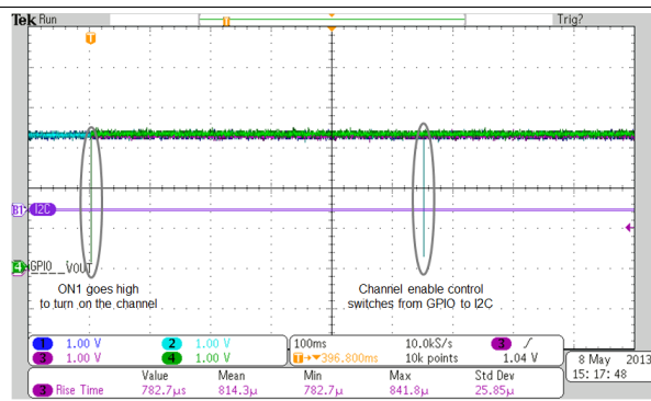
Figure 29. Channel 1 powered up via GPIO control, and control is switched over to I²C control without any glitches on VOUT.
