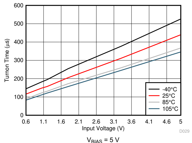
Figure 6-42. Turnon Time vs Input Voltage
