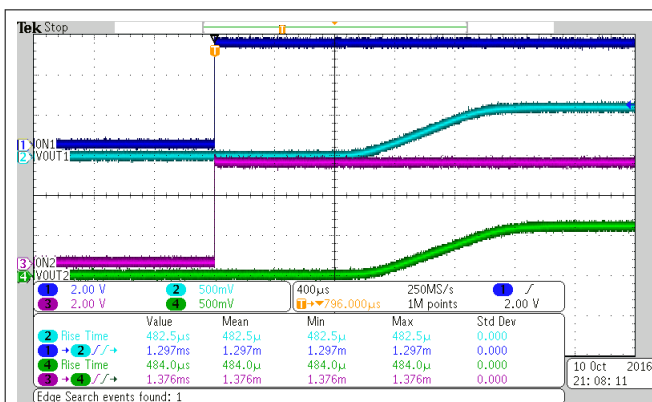
Figure 6-31. Turnon Response Time
