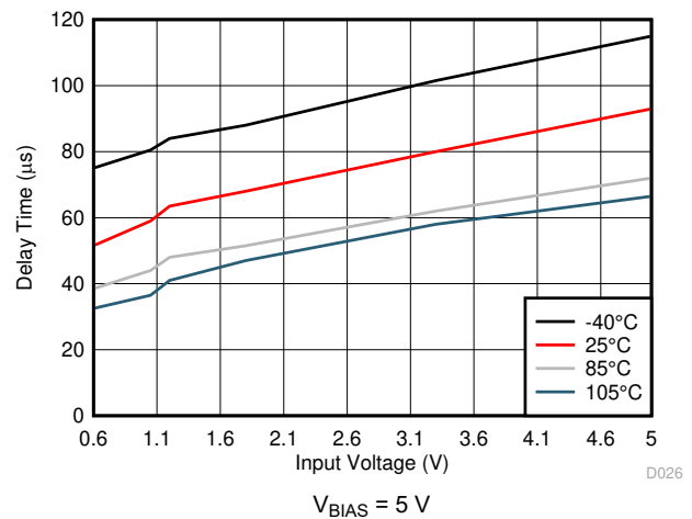
Figure 6-40. Delay Time vs Input Voltage
