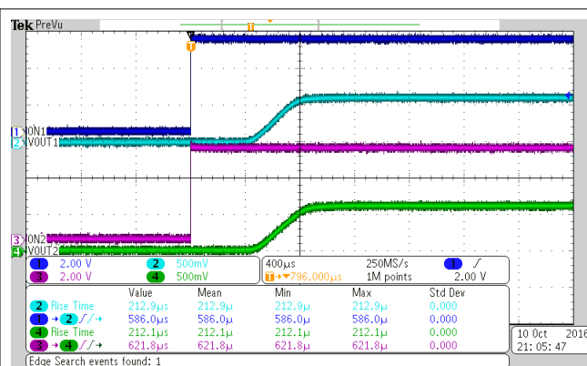
Figure 6-32. Turnon Response Time
