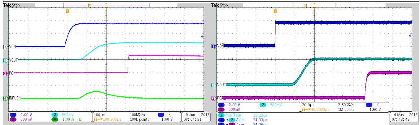
Figure 19. High Inrush Current at 3.6 \text{ V}_{IN}
