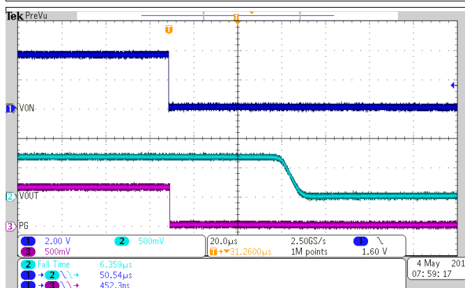
Figure 15. Turn-Off Response at 3.6 V_{IN}
