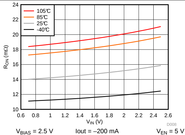
Figure 7. R_{ON} vs Temperature, V_{BIAS} = 2.5\text{ V}
