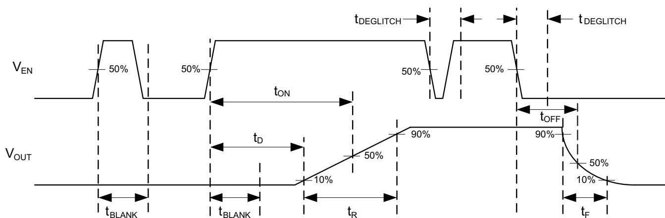
Figure 52. Timing Waveforms
