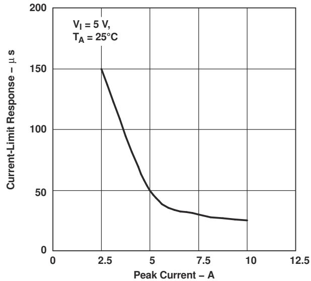
Figure 6-29. CURRENT-LIMIT RESPONSE vs PEAK CURRENT
