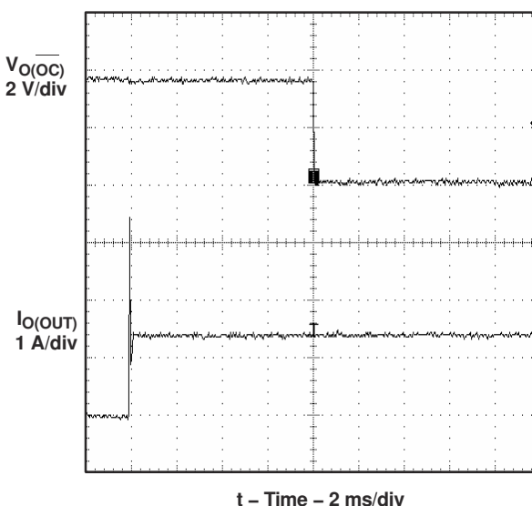
Figure 6-37. 1- \Omega Load Connected to Enabled Device
