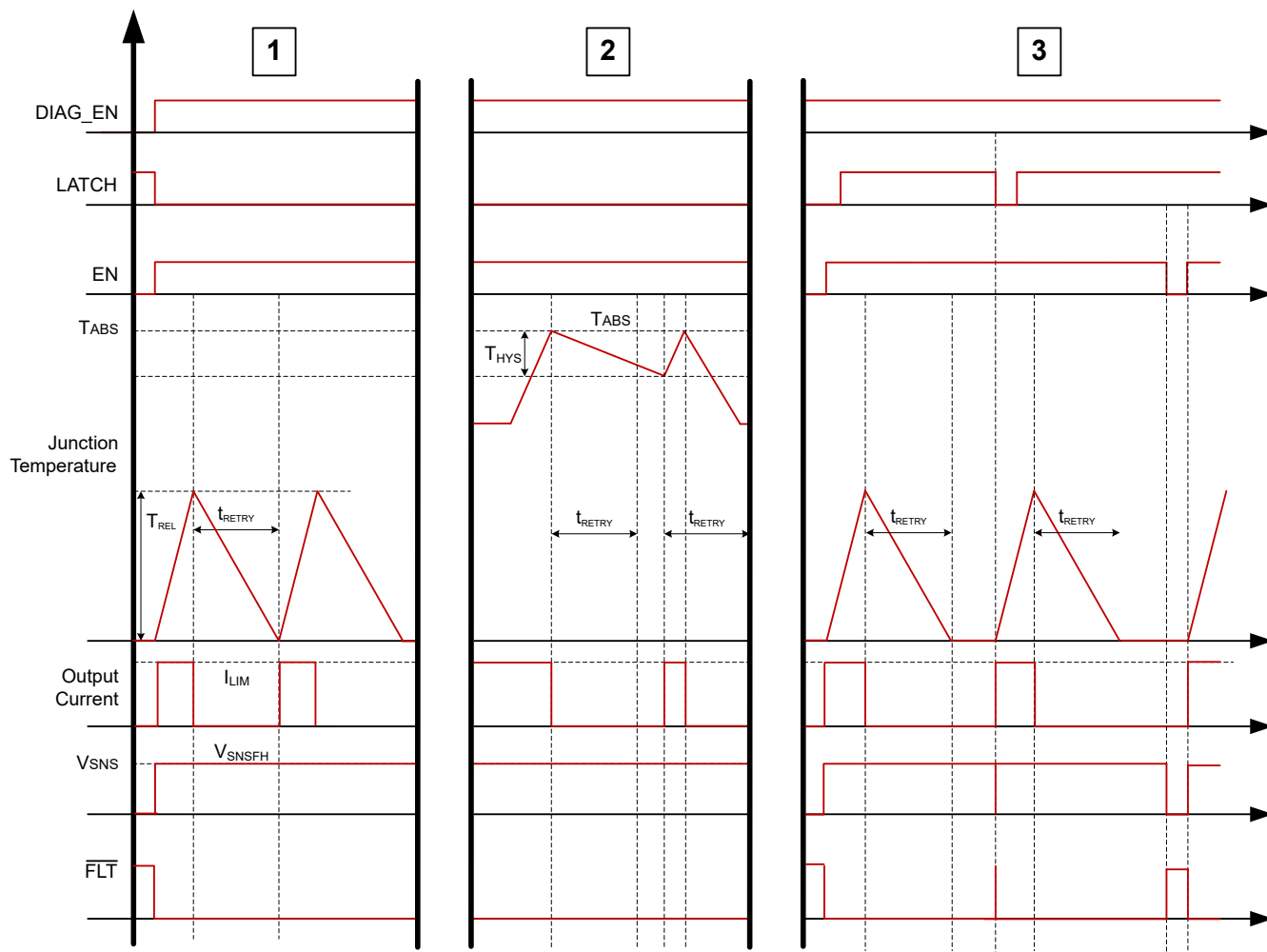
Figure 8-18. Thermal Behavior
