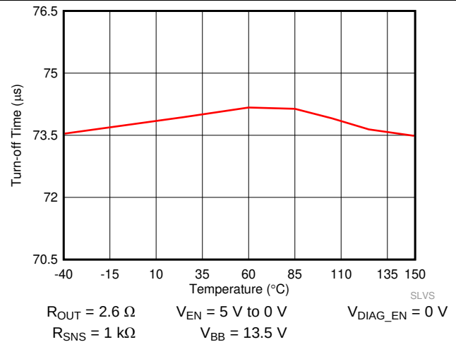
Figure 14. Turn-off Time ( t_{\text{OFF}} ) vs Temperature
