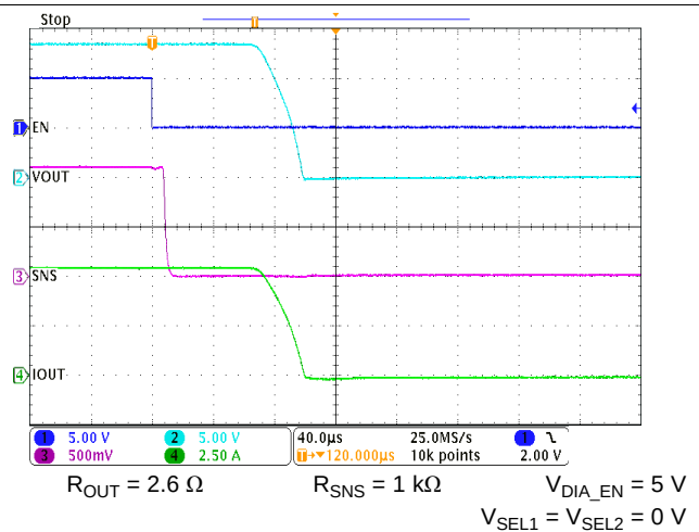
Figure 30. Turn-off Time ( t_{OFF} ) and Sense Settle Time ( t_{SNSION2} )
