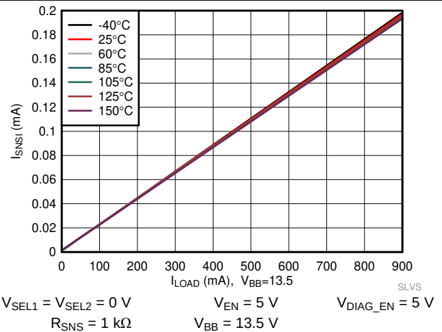
Figure 16. Current Sense Output Current ( I_{\text{SNSI}} ) vs Load Current ( I_{\text{OUT}} ) across Temperature
