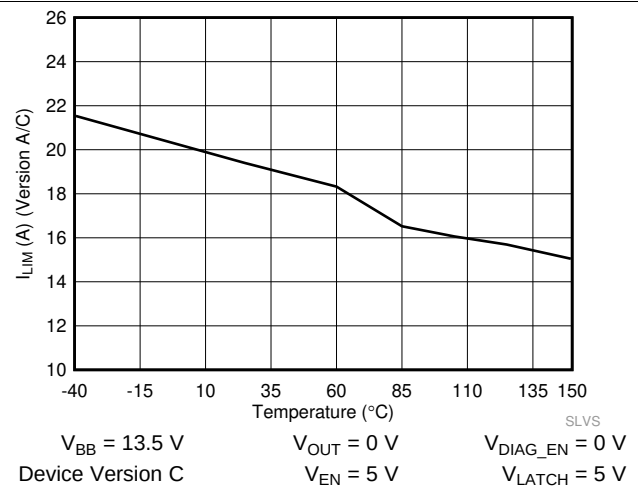
Figure 22. Current Limit ( I_{CL} ) vs Temperature
