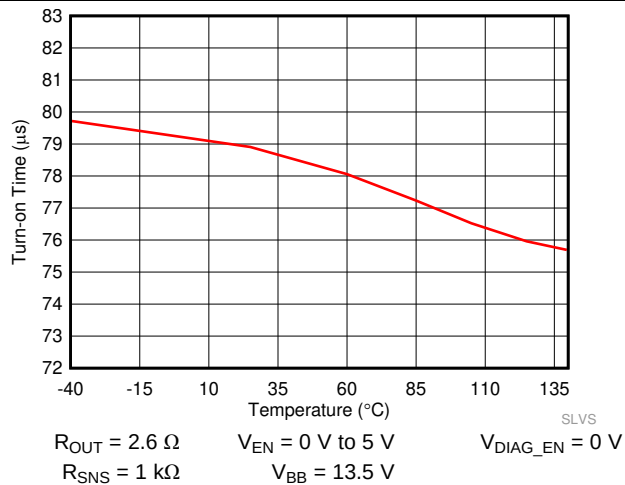
Figure 13. Turn-on Time ( t_{\text{ON}} ) vs Temperature
