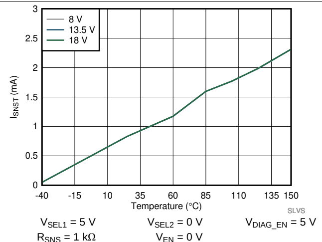
Figure 18. Temperature Sense Output Current ( I_{\text{SNST}} ) vs Temperature
