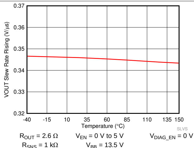
Figure 11. V_{OUT} Slew Rate Rising ( SR_P ) vs Temperature
