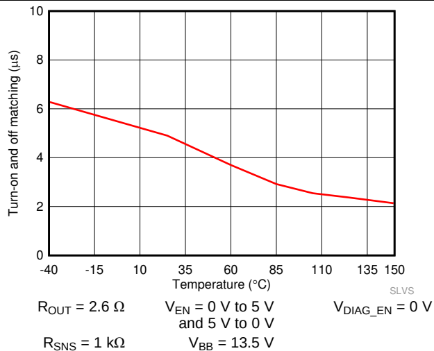
Figure 15. Turn-on and Turn-off Matching ( t_{\text{ON}} - t_{\text{OFF}} ) vs Temperature
