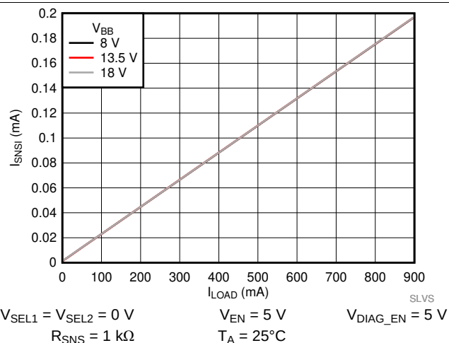
Figure 17. Current Sense Output Current ( I_{\text{SNSI}} ) vs Load Current ( I_{\text{OUT}} ) across V_{\text{BB}}
