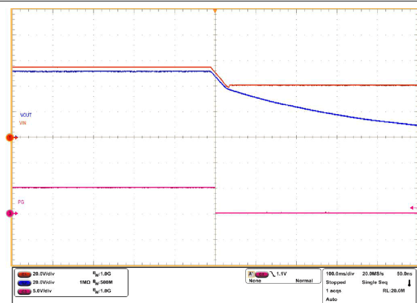
Figure 7-8. Undervoltage protection
