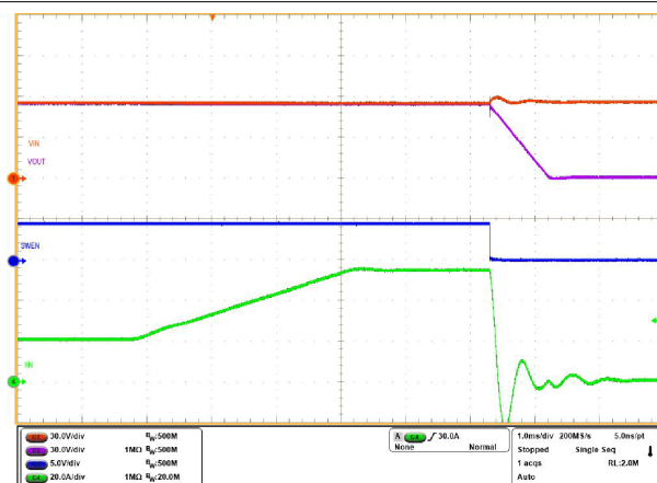
Figure 7-9. Overcurrent protection
