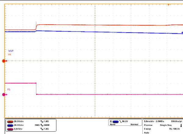
Figure 7-7. Overvoltage protection
