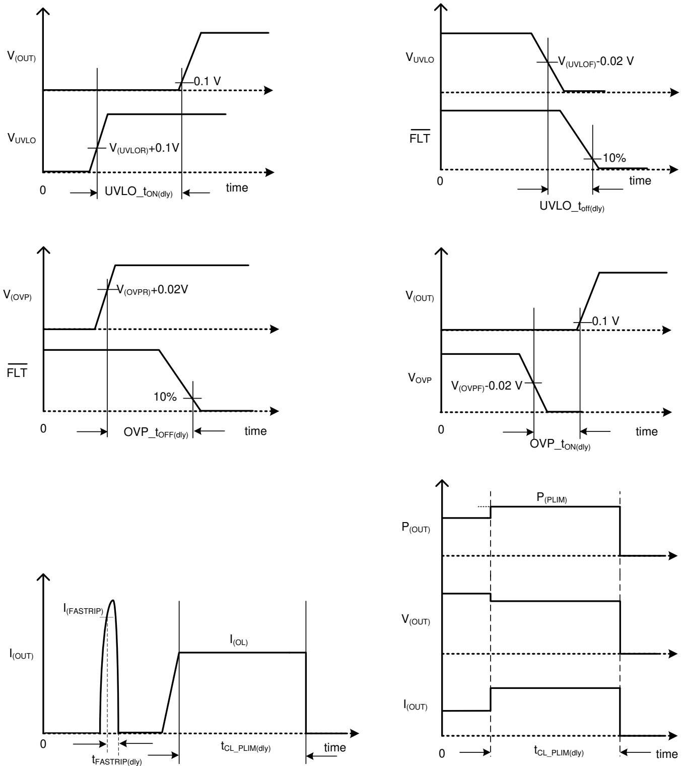
Figure 8-1. Timing Waveforms
