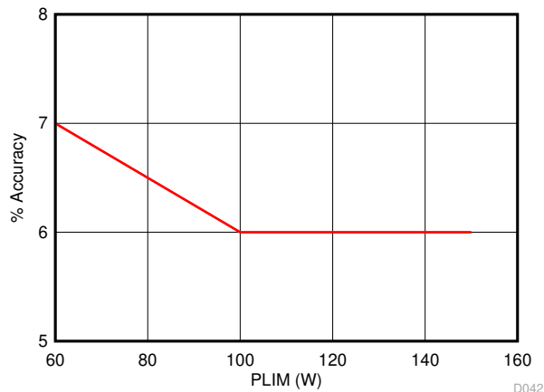
Figure 7-7. Output Power Limiting Accuracy vs PLIM
