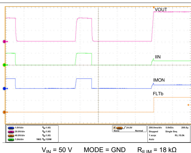
Figure 9-7. Coming Out of Overload With Load Step from 40 \Omega to 140 \Omega
