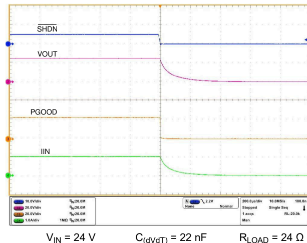
Figure 9-14. Turnoff Control With \overline{\text{SHDN}}
