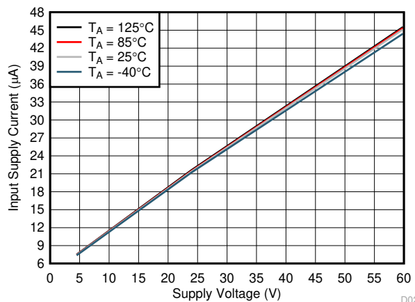
Figure 7-3. Input Supply Current vs Supply Voltage in Shutdown
