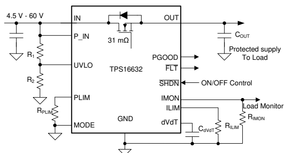
Simplified Schematic
