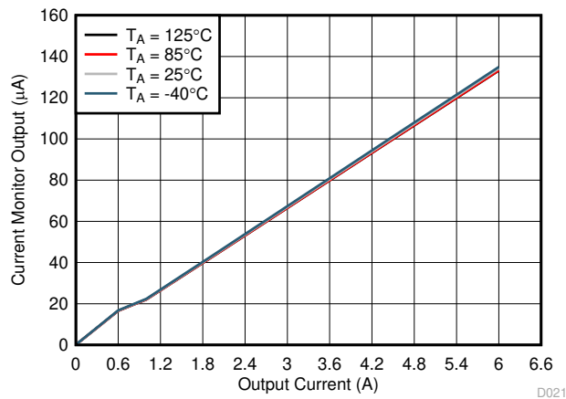
Figure 7-9. Current Monitor Output vs Output Current
