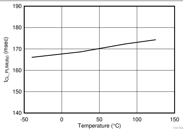
Figure 7-11. Maximum Duration in Current and Power Limiting vs Temperature
