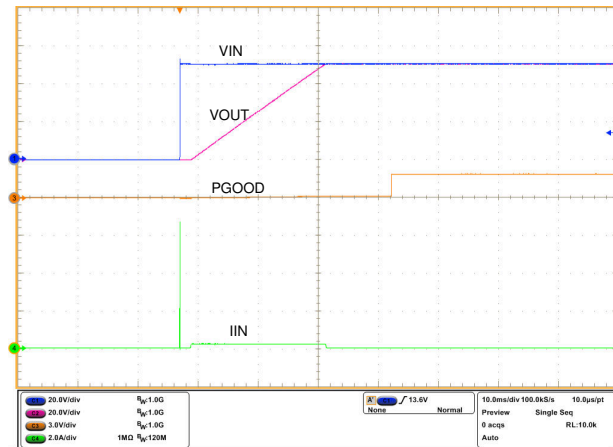
Figure 10-2. Hot-Plug In at 50-V Supply With No Load
