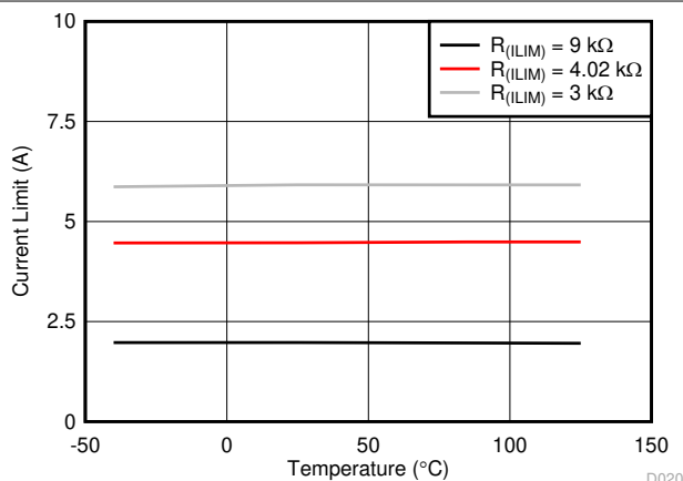
Figure 7-5. Overload Current Limit vs Temperature
