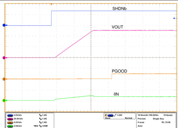
Figure 10-7. Turn ON Using SHDN Control
