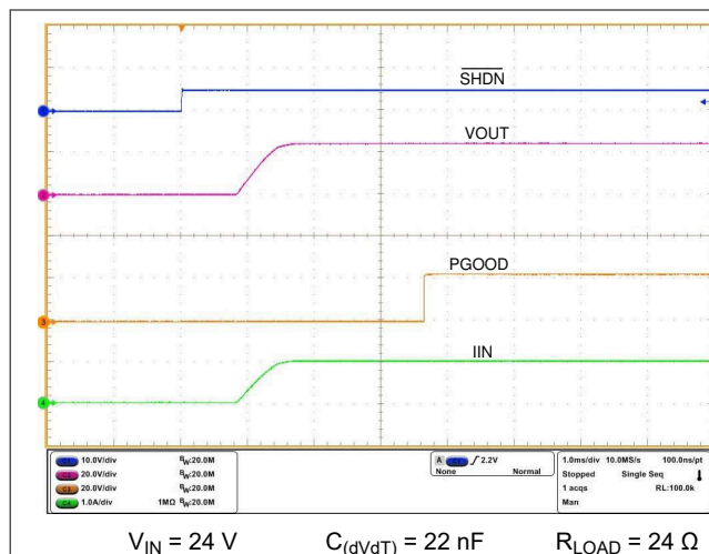
Figure 9-13. Turnon Control With \overline{\text{SHDN}}
