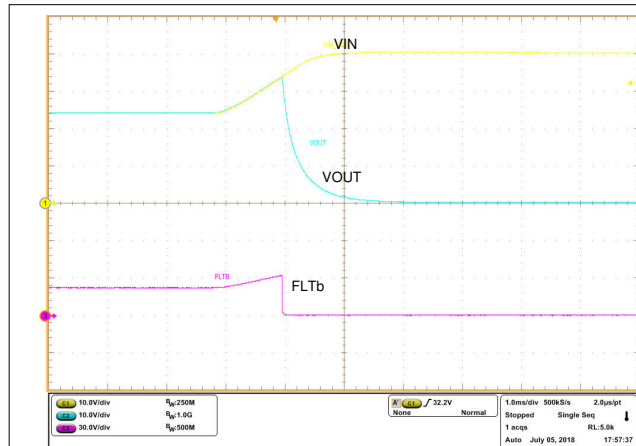
TPS16630 OVP Setting at 33 V Figure 9-4. Overvoltage Cut-Off Response at 33-V Level
