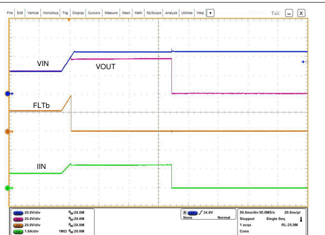
TPS16632 C_{OUT} = 10 \mu F , FLT connected to V_{OUT} R_{LOAD} = 30 \Omega Figure 9-5. Overvoltage Clamp Response
