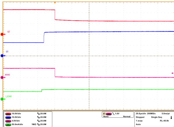
Figure 8-4. Zoom-In View of State Transition From LPM to Active Mode ( \overline{\text{LPM}} = \text{Low} , \text{VIN} = 12\text{V} , \text{EN}/\text{UVLO} = \text{High} )
