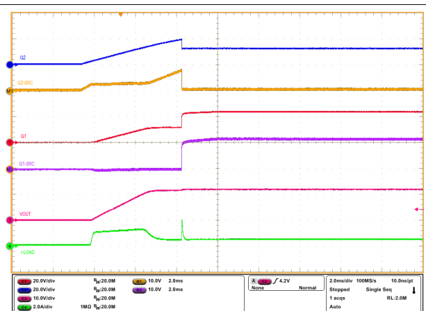
Figure 8-14. Inrush Current Profile with 220 \mu F at the Output and 0.5 A Load (LPM = Low)
