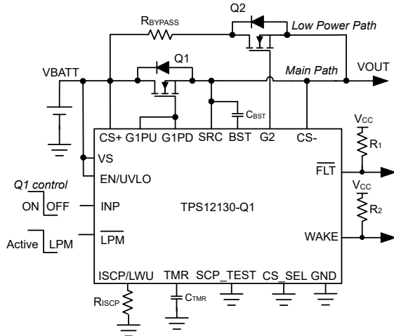
Figure 7-7. TPS12130-Q1 Application Circuit With Main FET RDSON Based Current Sensing
