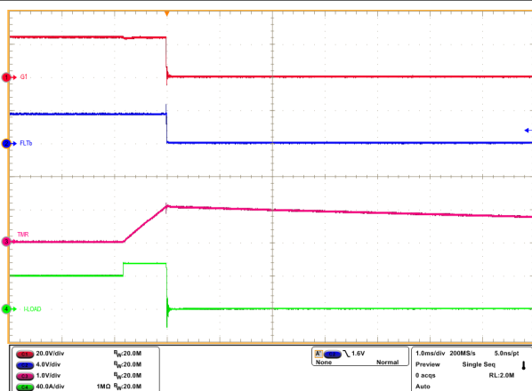
Figure 8-8. Overcurrent Response of TPS1213-Q1 EVM for 40A to 55A Load Step
