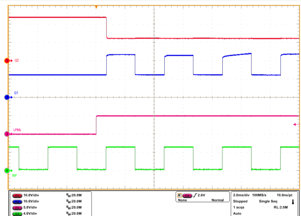
Figure 8-7. With LPM = Low to High, INP Gained Control on G1 (VIN = 12V, No Load)
