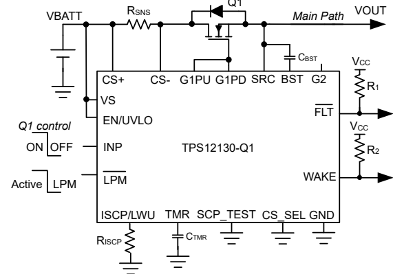
Figure 7-8. TPS12130-Q1 Application Circuit With External Sense Resistor R_{SNS} Based Current Sensing
