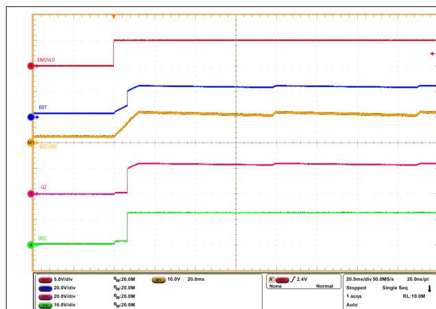
Figure 8-2. Start-Up Profile of Low Power Path (LPM = Low, VIN = 12V, No Load, CBST = 470nF)
