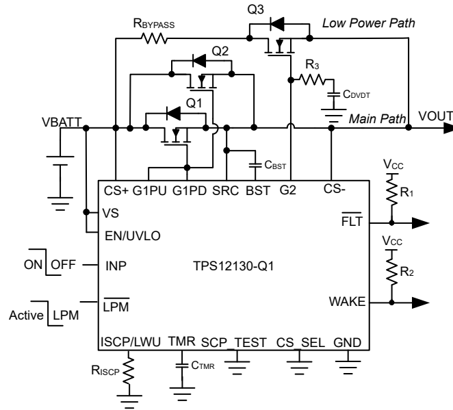
Figure 7-4. TPS1213-Q1 Application Circuit for Capacitive Load Driving Using Low Power Bypass FET and Series Power Resistor ( R_{\text{BYPASS}} )
