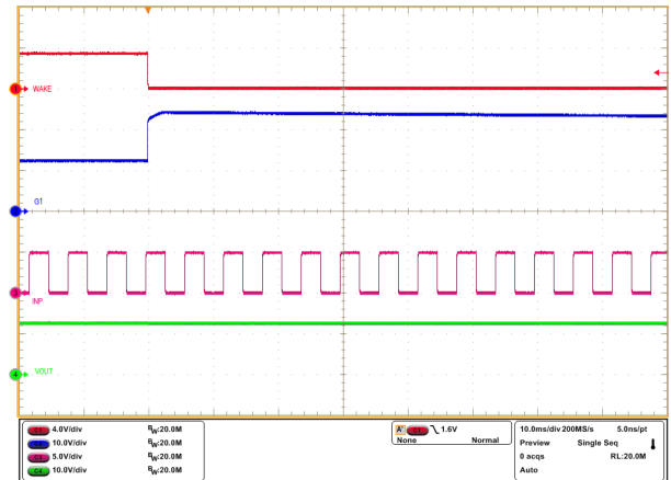
Figure 8-5. As \overline{\text{LPM}} = \text{Low} , INP Has No Control on G1 Even After WAKEUP
