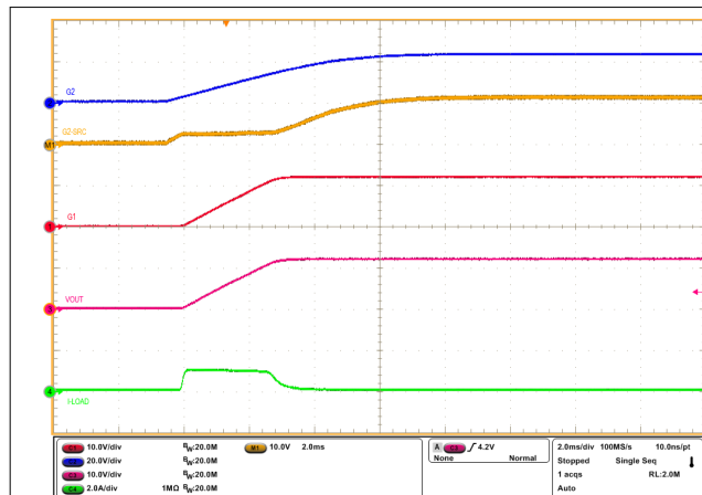
Figure 8-13. Inrush Current Profile with 220 \mu F at the Output (LPM = Low)
