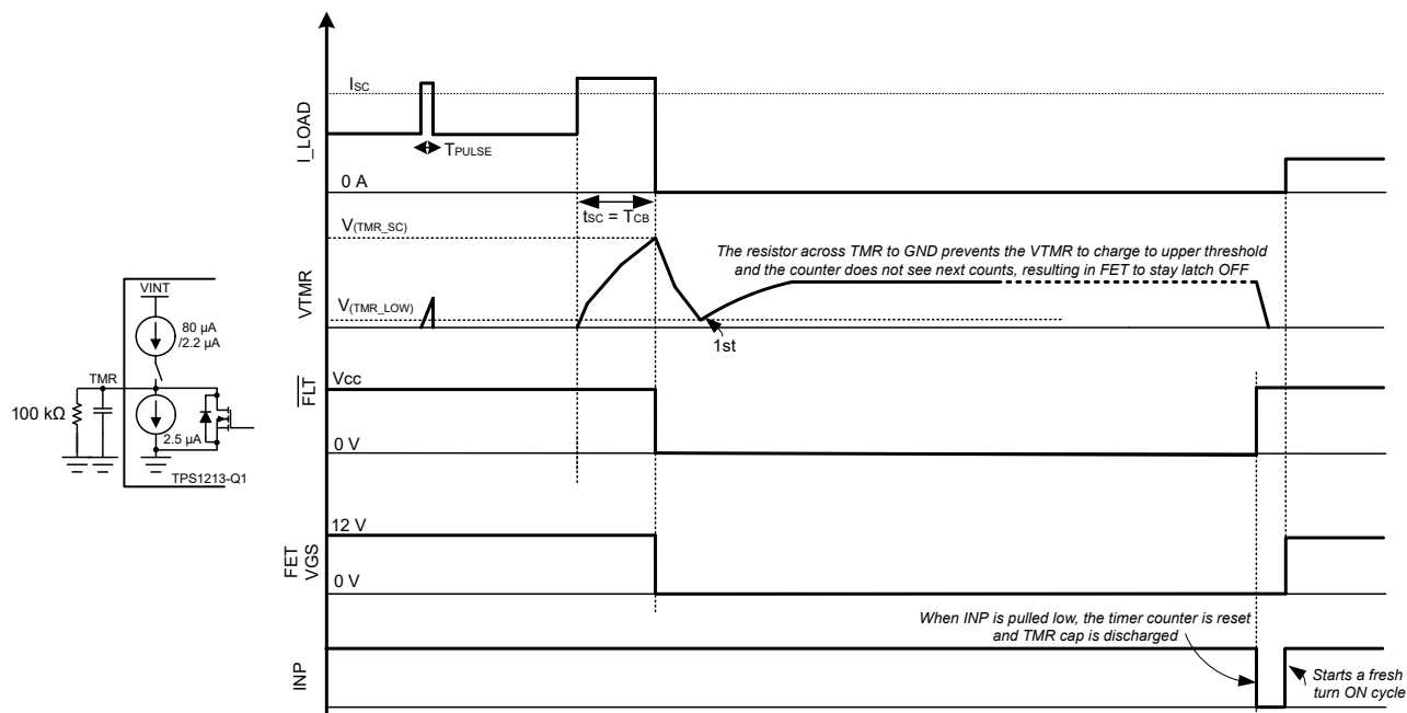
Figure 7-10. Short-Circuit Protection With Latch-Off
