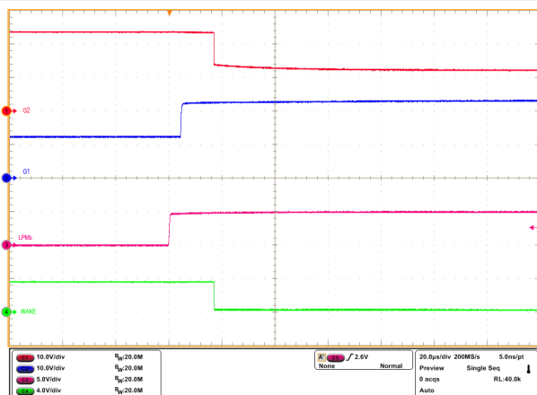
Figure 8-6. State Transition From LPM to Active Mode (LPM = Low to High, VIN = 12V, No Load)
