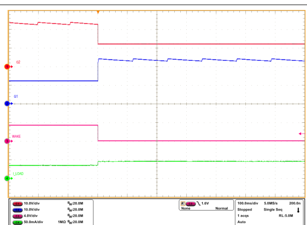
Figure 8-3. State Transition From LPM to Active Mode (LPM = Low, VIN = 12V, EN/UVLO = High)
