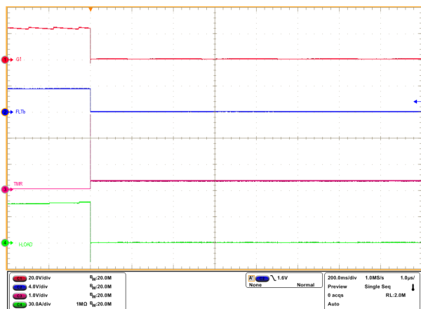
Figure 8-10. Latch-Off Response of TPS1213-Q1 for an Overcurrent Fault
