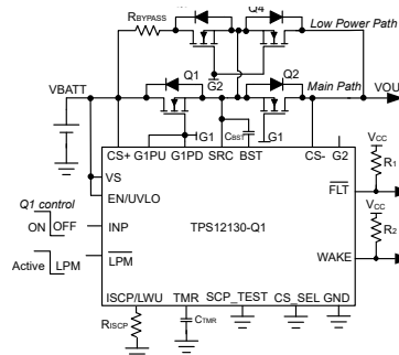
Always ON Automotive e-Fuse Driving Back to Back FETs
