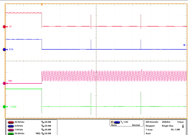
Figure 8-9. Auto-Retry Response of TPS12130-Q1 for an Overcurrent Fault
