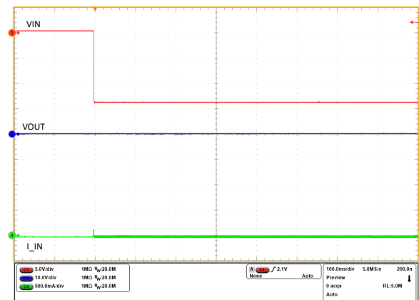
Figure 9-15. Input Reverse Polarity Protection with TPS12110-Q1
