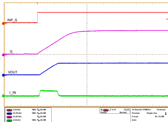
Figure 9-11. Precharge Profile of the Output Capacitance (VIN = 12 V, COUT = 1 mF, No Load)
