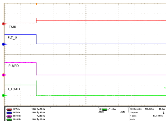
Figure 9-9. Latch-Off Response of TPS1211-Q1 for an Overcurrent Fault
