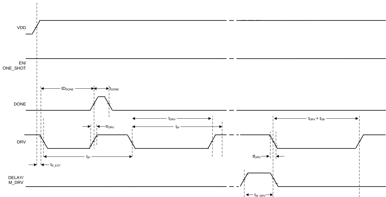
Figure 1. TPL5110 Timing
