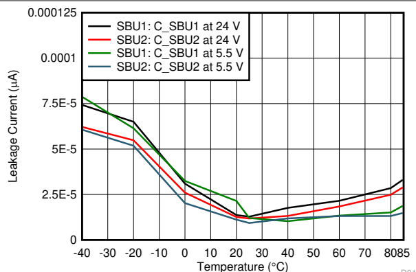
Figure 7-12. SBU OVP Leakage Current vs Ambient Temperature at 5.5 V and 24 V
