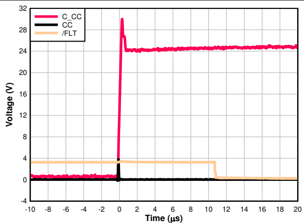
Figure 7-18. CC Short-to-V BUS 24 V Zoomed Out
