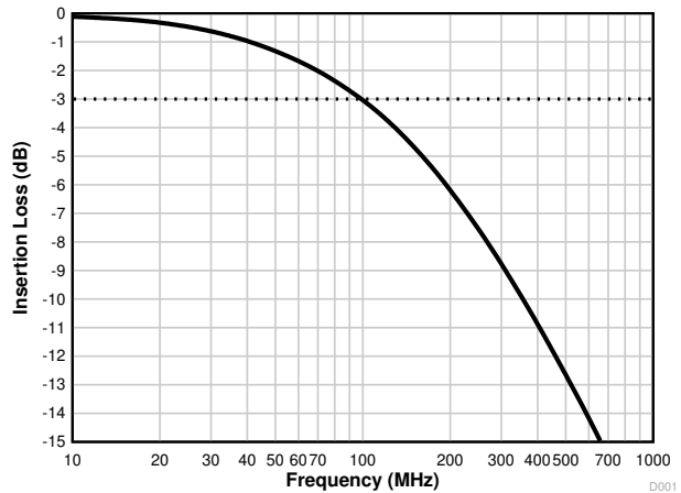
Figure 7-16. CC Bandwidth
