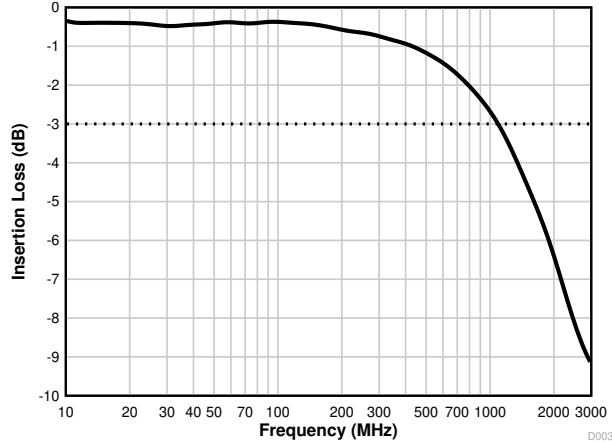
Figure 7-1. SBU Bandwidth
