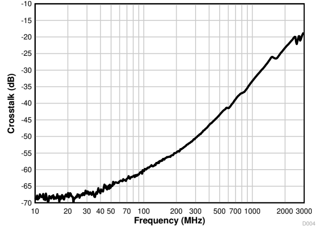
Figure 7-2. SBU Crosstalk
