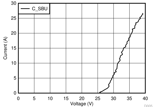
Figure 7-14. C_SBU TLP Curve Unpowered
