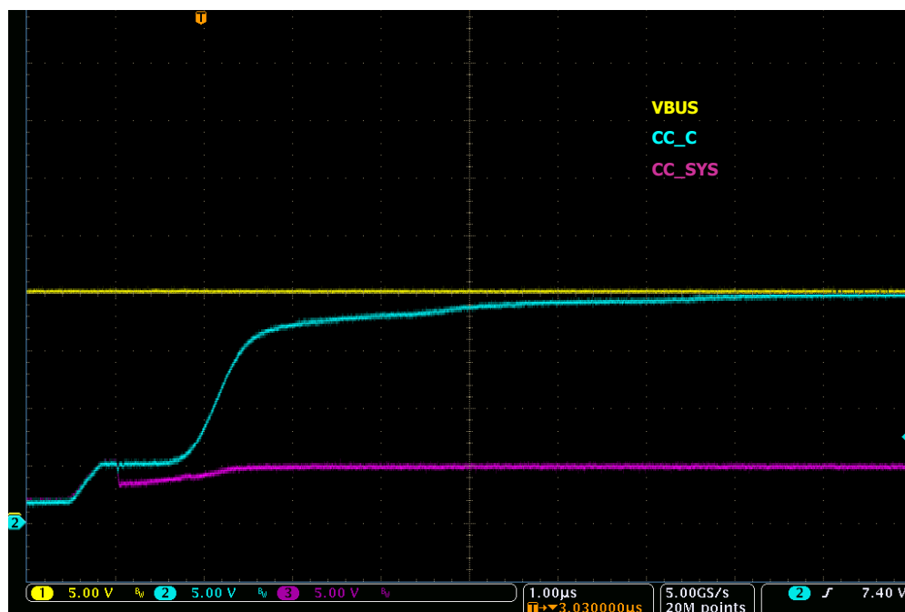
Figure 7-4. Short to VBUS Protection Example
