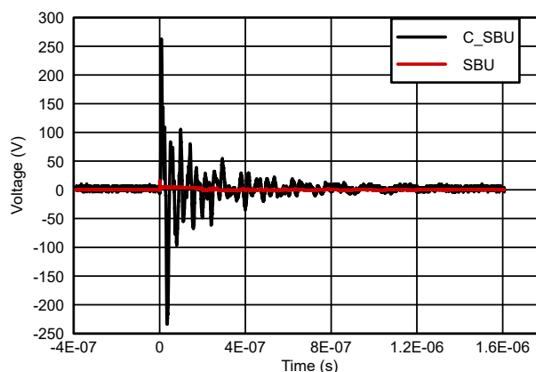
Figure 5-2. SBU IEC 61000-4-2 4kV Response Waveform
