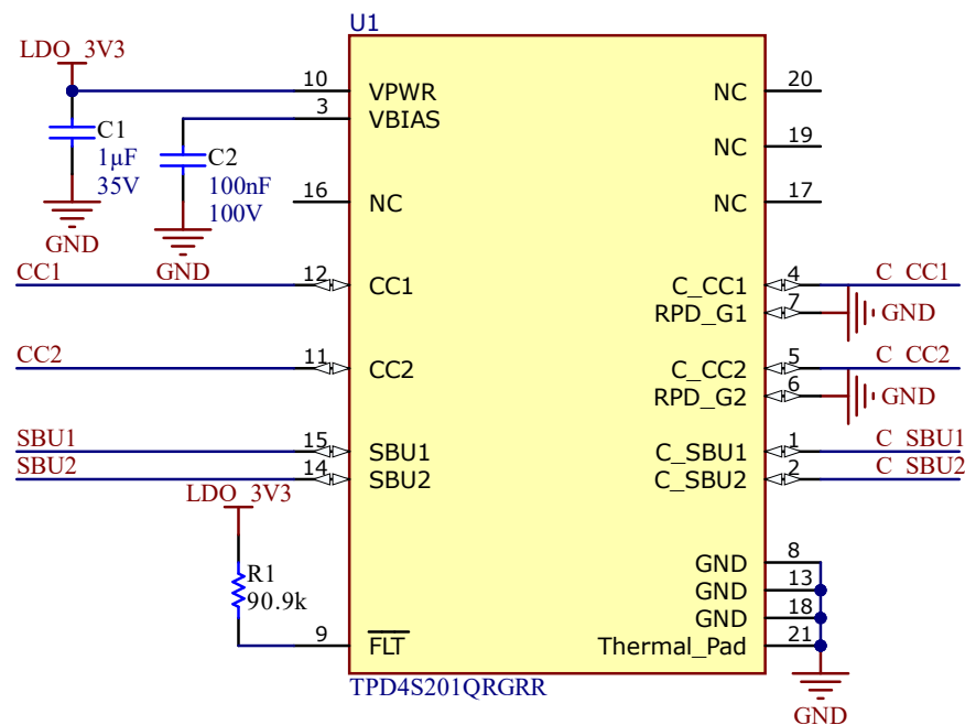
Figure 7-1. TPD4S201-Q1 No Dead Battery
