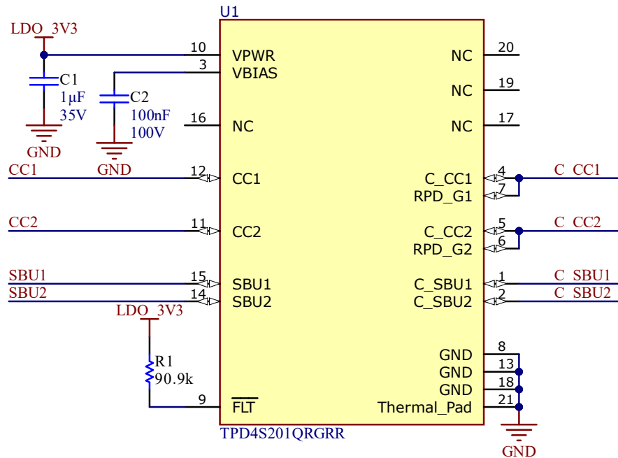
Figure 7-2. TPD4S201-Q1 Dead Battery
