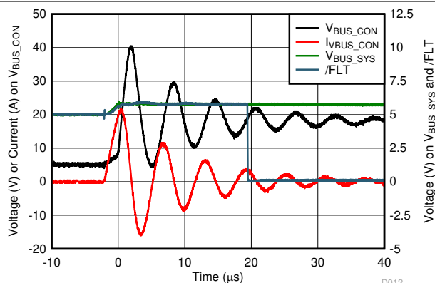
Figure 6-10. V_{\text{BUS}} Short-to-18 V Response Waveform
