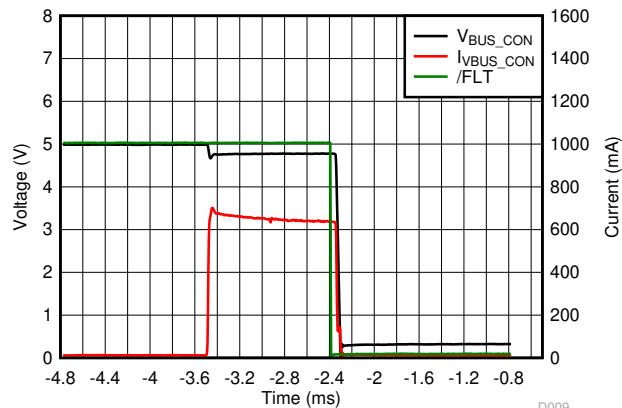
Figure 6-7. Overcurrent t_{\text{BLANK}} Response Waveform
