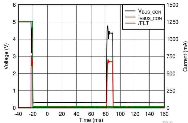
Figure 6-8. Overcurrent t_{\text{BLANK\_RETRY}} Response Waveform
