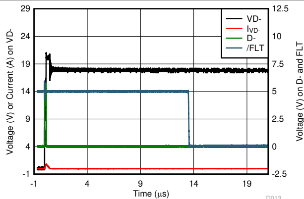
Figure 6-13. Data Switch Short-to-18 V Response Waveform (Long)
