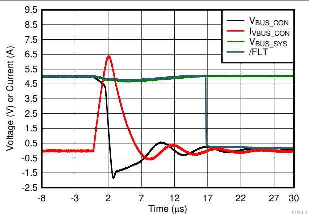
Figure 6-9. V_{\text{BUS}} Short-to-Ground Response Waveform
