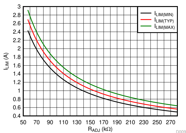
Figure 8-1. TPD3S716-Q1 Current Limit Thresholds vs. R_{ADJ}
