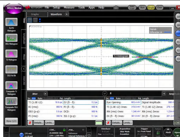
Figure 5-6. Jitter Decomposition of 20Gbps PRBS-7 Signals in TI Evaluation Board Through a Typical TMUXHS4412 Channels
