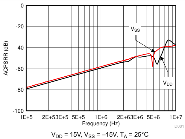
Figure 5-16. ACPSRR vs Frequency
