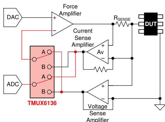
Figure 7-3. FVMC Implementation in PMU Using the TMUX6136
