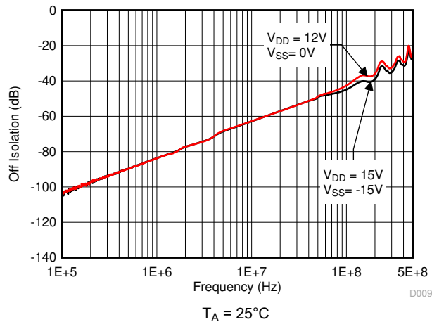
Figure 5-9. Off Isolation vs Frequency
