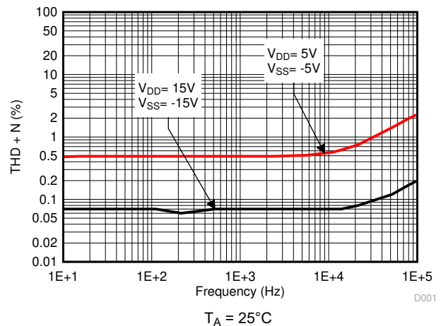
Figure 5-12. THD+N vs Frequency
