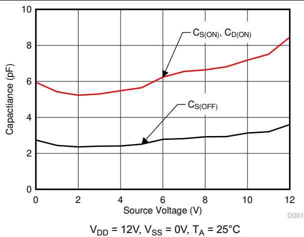
Figure 5-15. Capacitance vs Source Voltage
