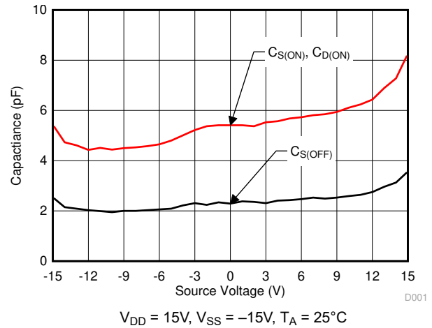
Figure 5-14. Capacitance vs Source Voltage
