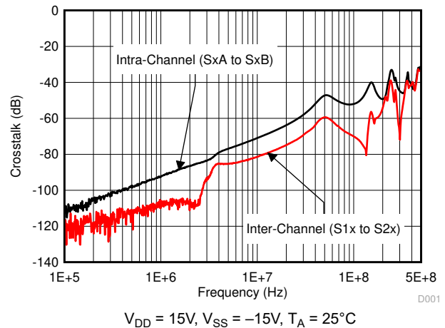
Figure 5-10. Crosstalk vs Frequency
