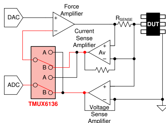
Figure 7-4. FCMV Implementation in PMU Using the TMUX6136
