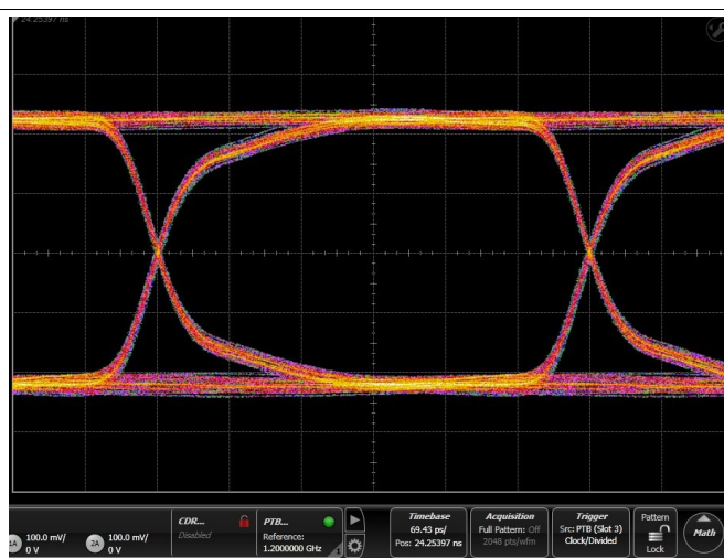
T_A = 25^\circ\text{C} Bias = 1.5 V 50 \Omega Termination Figure 26. Eye Pattern: 2.4 Gbps Through Path
