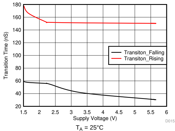
Figure 15. T_{TRANSITION} vs Supply Voltage
