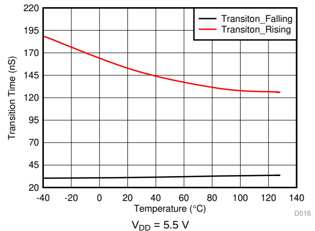
Figure 16. T_{TRANSITION} vs Temperature
