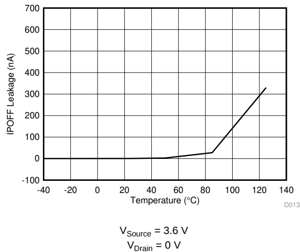
Figure 13. IPOFF Leakage vs Temperature
