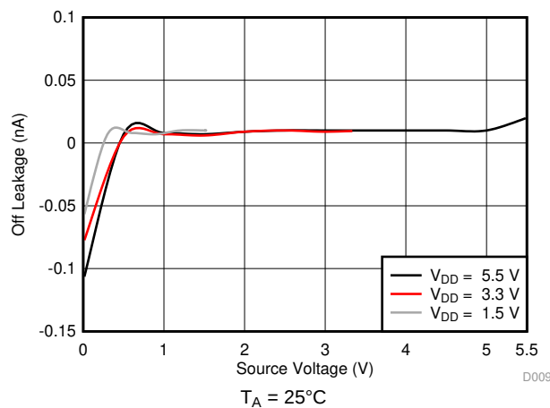
Figure 9. Off-Leakage vs Source or Drain Voltage
