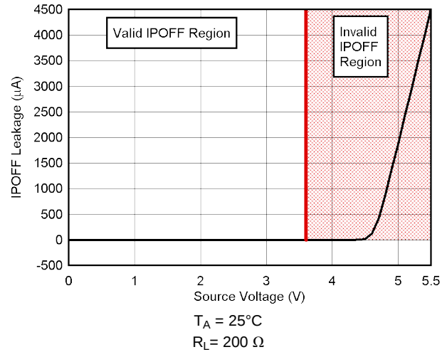
Figure 14. IPOFF Leakage vs Source or Drain Voltage
