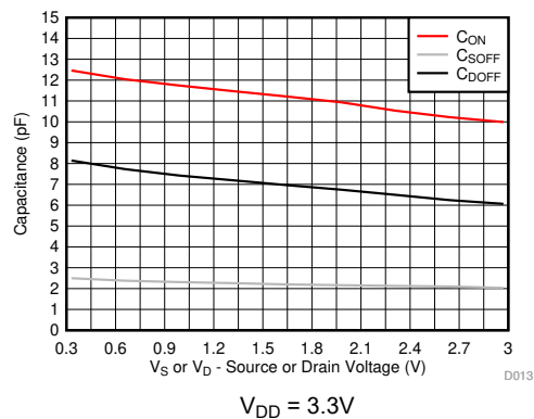
Figure 6-6. Capacitance vs Source Voltage
