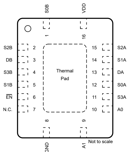
Figure 5-6. TMUX1309A: BQB Package, 16-Pin WQFN (Top View)
