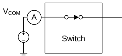
Figure 6. On Leakage
