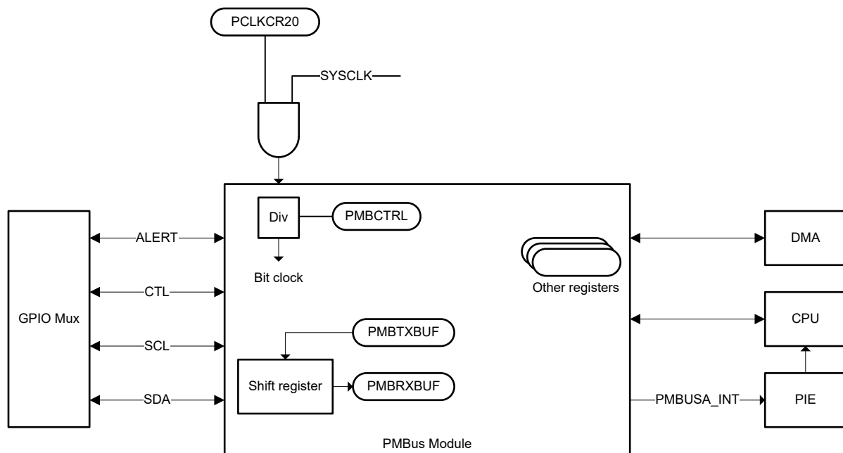
Figure 6-96. PMBus Block Diagram
