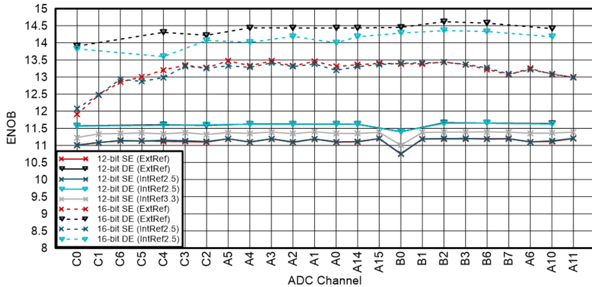
Figure 6-53. Per-Channel ENOB for 100-Pin PZP
