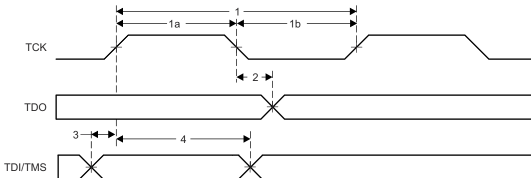
Figure 7-18. JTAG Timing
